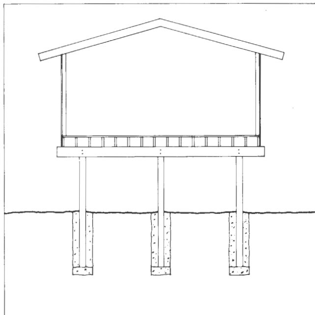
Figure 4.28. Platform Construction
