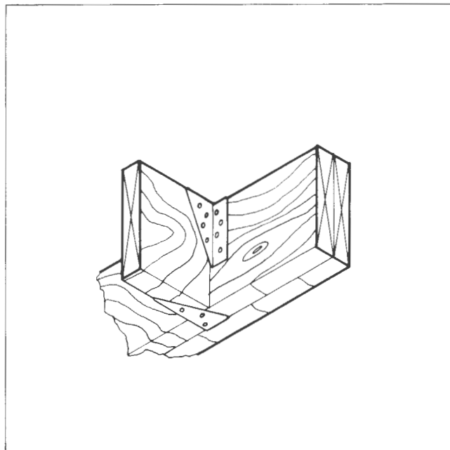
Figure 4.27. Metal Framing Anchors
